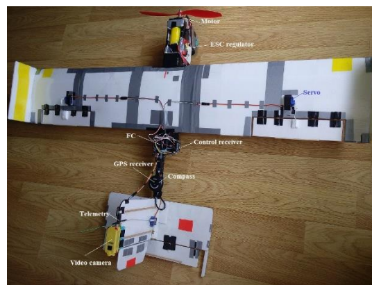
Figure 1 The photo of the tested aircraft.
