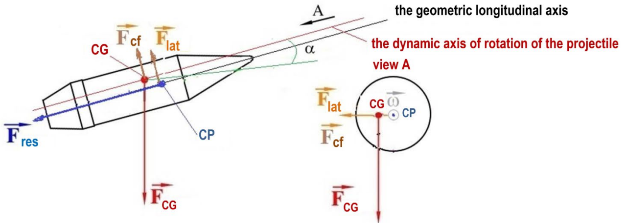
Figure 4. Location of forces when the CG and CP do not coincide and the CG is on the dynamic axis of rotation of the projectile, and the CP is on the geometric longitudinal axis, which do not coincide
